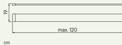
Murano estante y toallero Murano shelf and towel rail No compatible con Ala abatible. Para cristales máximo 120cm Not compatible with Swing wing. For fixed glass maximum 120cm
